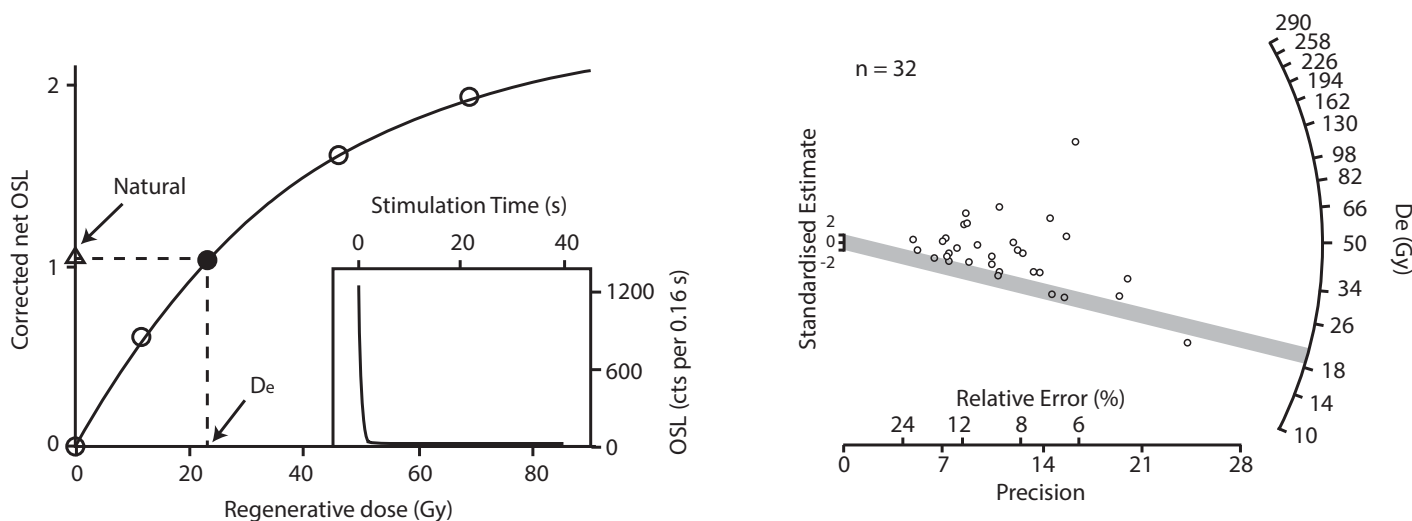
Figure 4. Optically stimulated luminescence plots for sample OSL-PKV-2. Sample was collected from a Qa 3 silt lens (see Fig. 2A for location) at 1.1 m vertical depth on a freshly incised ~2.5-m-high stream bank. A calibration growth curve (above left) illustrates the typical sensitivity corrected luminescence signal as a function of laboratory-induced regenerative dose (Gy) for a single aliquot. The filled circle is luminescence data for a repeated regenerative dose at the end of the measurement cycle; a value of unity in the ratio of these replicated measurements indicates correction of any luminescence sensitivity change throughout a measurement sequence. The equivalent dose, D_e , is found by interpolation of the natural luminescence signal with the regenerative-dose growth curve. An inset decay signal plot reveals a strong ~1200 initial count with a fast decay when exposed to a blue diode light source, indicative of good quartz sensitivity. The radial plot (above right) shows the D_e in values of grays (e.g., Galbraith, 1990), for 32 aliquots, as a function of its relative error and precision. Samples plotting to the right are more precise and have lower relative error. D_e is the effective amount of environmental radiation received since bleaching and deposition. The shaded bar on radial plot fits a 2\sigma uncertainty space through the five aliquots, comprising the minimum age model, to estimate a representative D_e for the sample. A minimum age model is appropriate here (Galbraith et al., 1999) because of the over dispersion and asymmetrical population of D_e values measured (~61%), characteristic of incomplete bleaching of quartz grains during transport. An aliquot plotting below this bar is treated as an outlier, and thus not used to determine a bulk D_e for OSL-PKV-2. Table 3 in the text gives a separate summary of the dating information. Data Repository item DR1 (see footnote 1) provides summary of methodology used.
