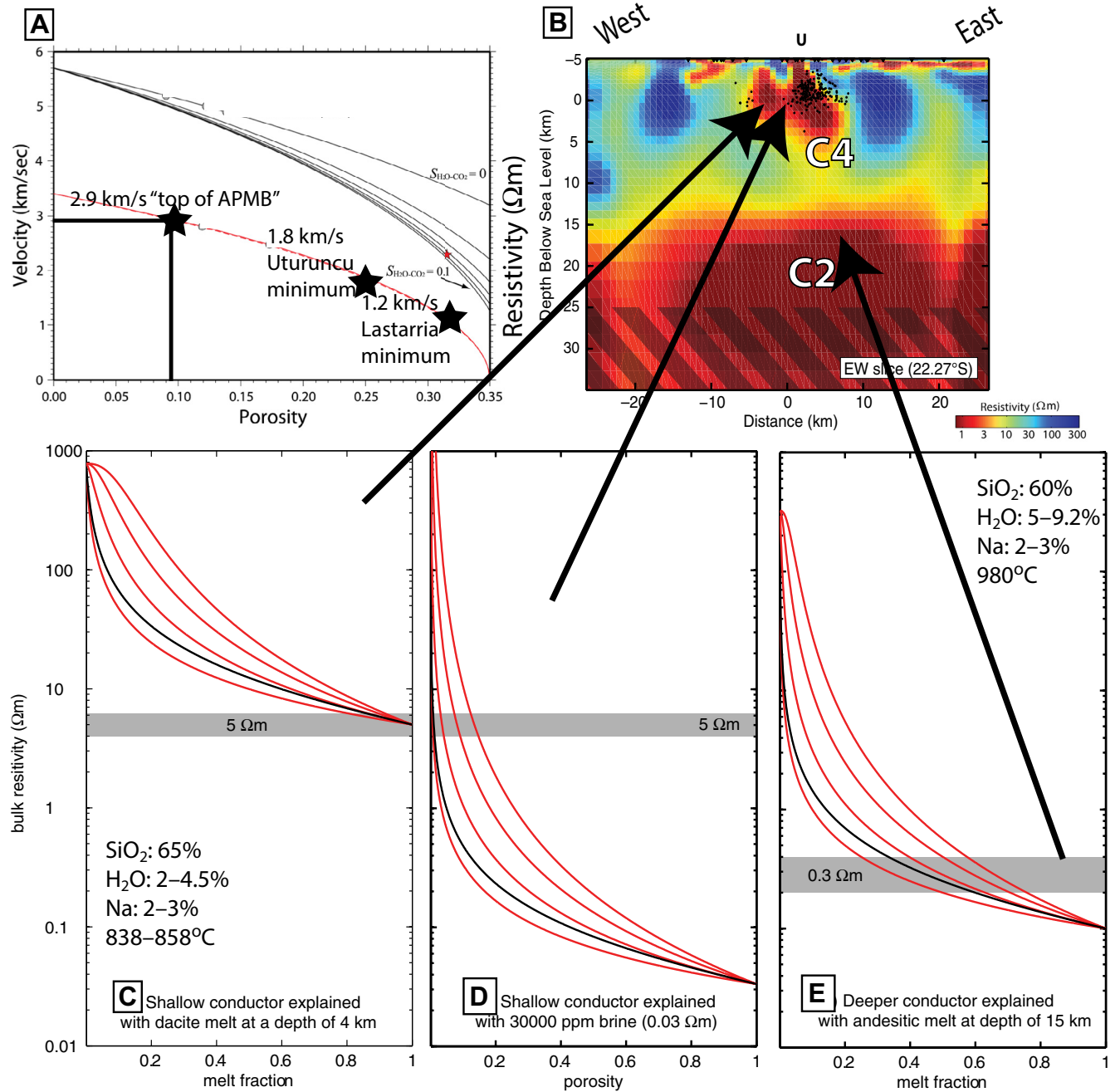
Figure 6. Geophysical inferences of the amount of subsurface melt and/or fluid. (A) Conversion of V_p and V_s to porosity (partial melt plus volatile phase) from Chu et al. (2010). The plot shows the V_s values that were used to define the limits of “significant partial melt” (2.9 km/s, ~10% partial melt, Ward et al., 2014b), the minimum V_s seen beneath Uturuncu in the Altiplano-Puna Magma (or Mush) Body (APMB) (1.8 km/s, implying 25% partial melt) and beneath Lastarria volcano (1.2 km/s, implying ~32% porosity) near the Lazufre deformation center. (B) The 3D resistivity model from Comeau et al. (2016) and (C–E) show variation of bulk resistivity as a function of the quantity of fluid all at Uturuncu. (C) Model predictions of bulk resistivity of the shallow low-resistivity region from dacite melt using the chemical composition of the melt (Comeau et al., 2015). The gray bar shows the observed value from the model in (B) which can only match the models at unrealistically high melt fraction. (D) Model prediction of bulk resistivity from the same region as (C) from a mix of aqueous fluids and dacite. A porosity <5% of interconnected salty aqueous fluids is needed to explain the observed resistivity. (E) Bulk resistivity of the deeper low-resistivity feature modeled with andesite melt having resistivity of 0.1 \Omega\text{m} (Comeau et al., 2015). In C, D, and E, the red curves use a modified Archie’s Law with cementation exponents of 1, 1.5, 2, and 2.5. The black curve shows the Hashin-Shtrikman upper bound, and represents well-interconnected fluids.
