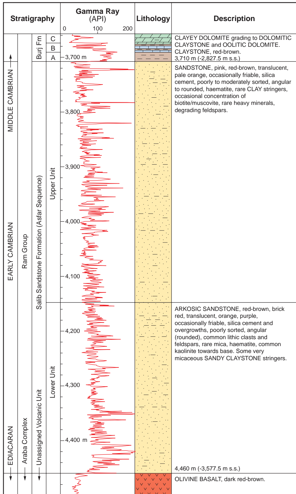
Figure 4: Reference section of Salib Formation in Wadi Sirhan-3 Well (WS-3) (after Andrews, 1991, reproduced by the permission of the Natural Resources Authority, Jordan). The 'Unassigned Volcanic Unit' is probably equivalent to the Aheimir Volcanic Suite.
