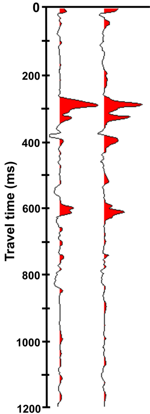
Fig. 6. Representative seismoelectric soundings on the West Greenland Ice Sheet. The two dominant seismoelectric arrivals at c. 305 ms and c. 610 ms were both generated at the ice-bed interface ( c. 1145 \pm 15 m; Booth et al. 2012; Kulesa et al. In review), and are consistent with a seismoelectric conversion and the arrival of co-seismic energy, respectively.
